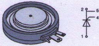
Thyristor
